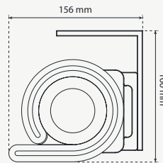
Ceiling Mounting
