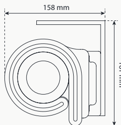
Ceiling Mounting
